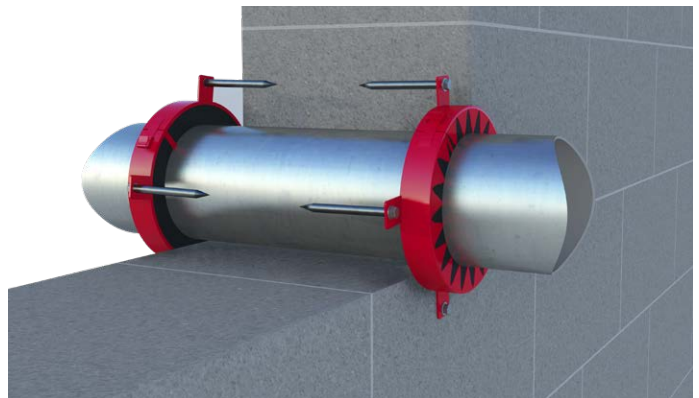
Pipe Collar CE wall application
