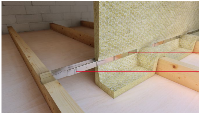
Figure 8 Barrier fitted transversely to timber joisted ceiling
