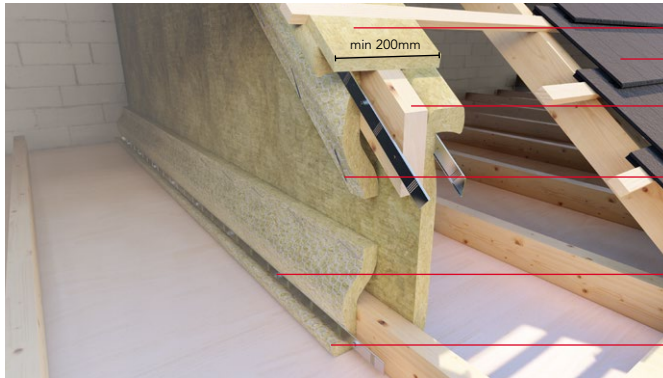
Figure 6 Half hour protection for timber truss construction 35 to 49mm thick.
