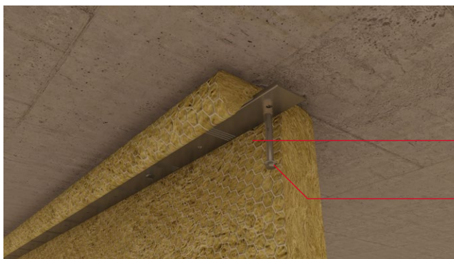
Figure 12 Alternative fixing to flat soffit or perimeter, appropriate to barriers with a shallow drop
