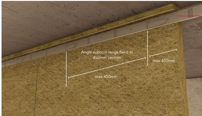
Figure 10 50mm Fire Barrier fixed to concrete soffit.
