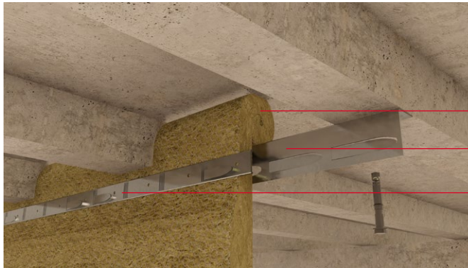
Figure 11 50mm Fire Barrier running across ribbed soffit - Section
